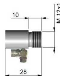
TM-AP-CS Air purge collar for 10:1 sensors
