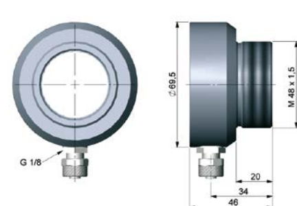
TM-AP-CTL Air purge collar
