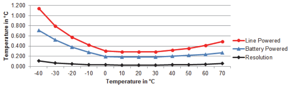
Plot A: Accuracy Range of ZW-003 Integrated Temperature Sensor
