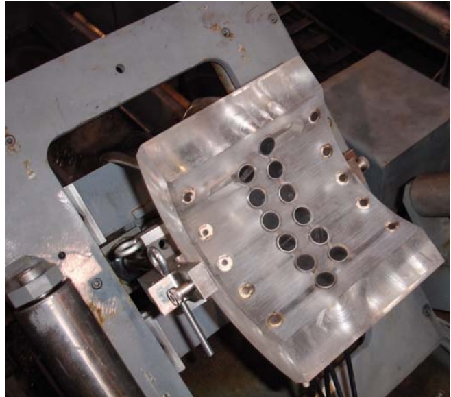
Test Head in Round Testing Configuration
