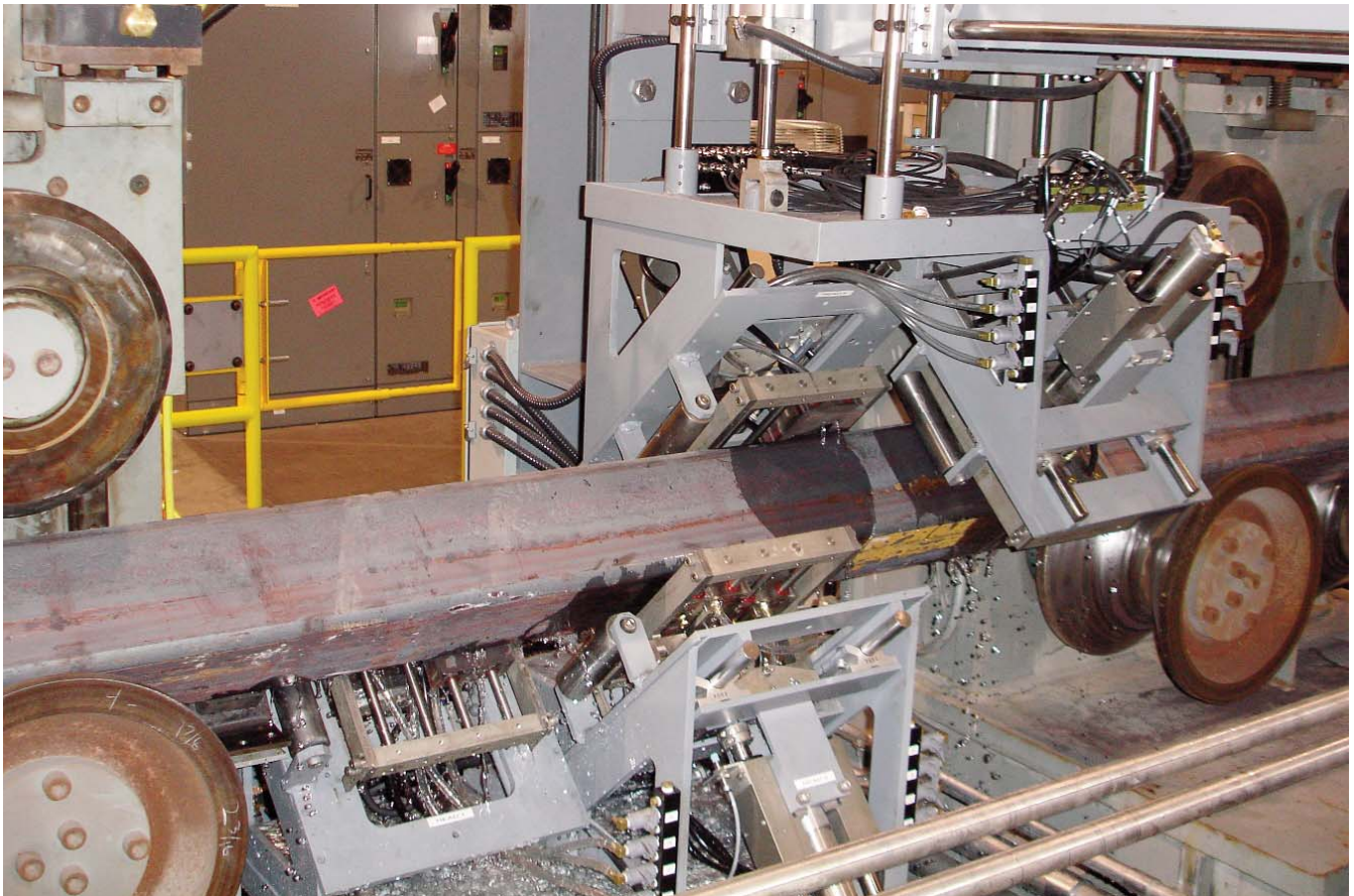
MAC Ultrasonic Billet Test System Inspecting 7" Diameter Square Billets
