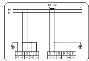
Single-phase connection
