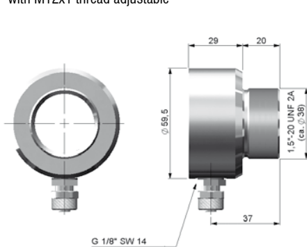
TM-AP-CX Air purge collar CX sensors
